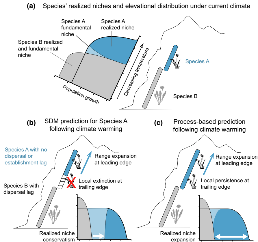
FIGURE 2 Range predictions for a focal alpine species (species A) following climate change. Species A shows a trade-off between population growth rate and tolerance of low temperature, such that it can tolerate a greater range of temperature than species B, but is outcompeted by species B under warmer climatic conditions (i.e. it has a broader fundamental niche than species B, but a realized niche restricted to cooler temperatures) (a). Following climate warming, a simple species distribution modelling (SDM) approach for species A, that assumes realized niche conservatism, would predict high elevation range expansion and low elevation range contraction (b). However, if species B is constrained by a dispersal lag, as shown, then the prediction of local extinction at the lower elevation range margin for species A would be incorrect. Instead species A would persist at its current lower elevation range margin, expanding its realized niche, due to the absence of competition from species B (c). This outcome would be predicted by process-based models that account independently for effects of climate and competition on population growth rates [Colour figure can be viewed at wileyonlinelibrary.com ]
