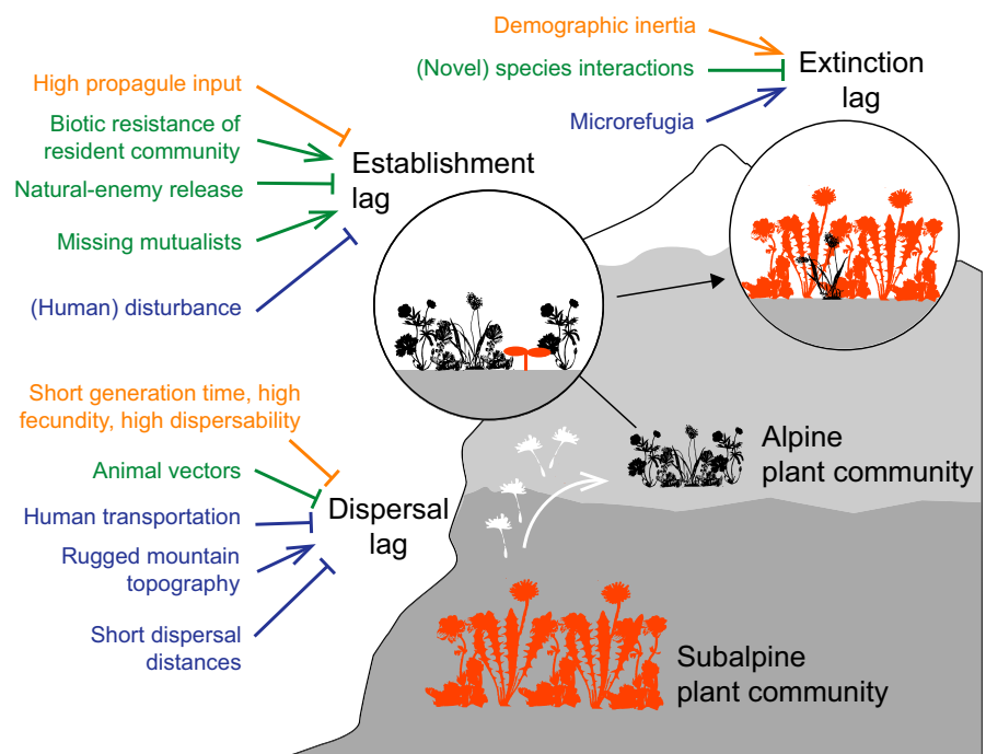
FIGURE 1 The magnitude and pace of alpine plant community turnover with climate change will be influenced by rates of species dispersal from lower elevations (“dispersal lags”), their rates of establishment and population growth in alpine communities (“establishment lags”) and extinction rates of resident alpine species (“extinction lags”). We include factors highlighted by our review that will increase (pointed arrows) or decrease (flat arrows) the magnitude of lags (factors related to focal species physiology and demography, biotic interactions, and the physical environment coloured orange, green and blue, respectively, in the online version) [Colour figure can be viewed at wileyonlinelibrary.com ]
