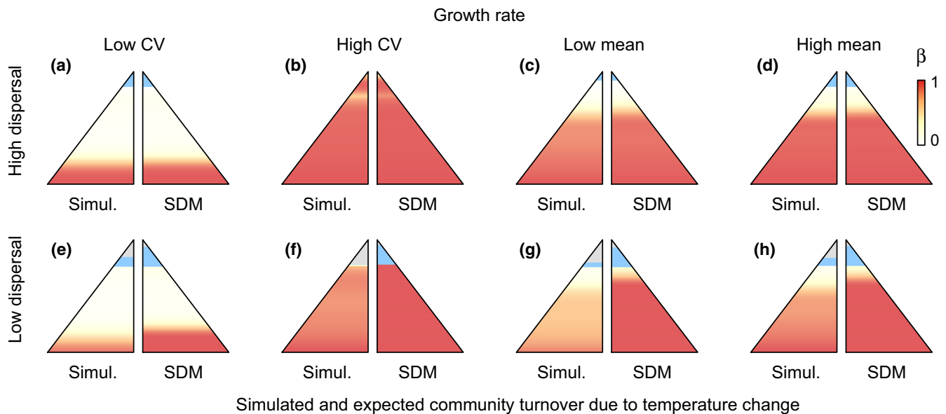
FIGURE 3 Temporal community turnover along an elevational temperature gradient ( \beta -diversity, represented by the gradient from white to red, see legend in (d)) following climate warming. The left section of the mountains represents the results of simulations (“Simul.”), while the right section represents the expected turnover obtained by simply stacking species distribution model projections (“SDM”). Shown are eight scenarios that differ depending on dispersal ability (rows) and growth rate within the species pool (a, e: coefficient of variation [CV] = 0.1; b, f: CV = 1/\sqrt{3} ; c, g: mean = 0.2; d, h: mean = 0.5; a–d: d = 10^{-1} ; e–h: d = 10^{-4} ). In each panel, all other parameters except the ones specified in the header of their line and column were set to the average value of their respective distribution (see Table S1). The lowest elevation communities are not displayed (see Appendix S1). Communities at the highest elevations resulting from colonization of previously unoccupied habitat are coloured in blue, while communities that remain empty despite warming are in light grey. Note that outcomes of temporal community turnover obtained from stacking SDM projections can also differ slightly among panels due to different initial conditions (i.e. initial burn-in period that allowed the meta-communities to equilibrate) [Colour figure can be viewed at wileyonlinelibrary.com ]
