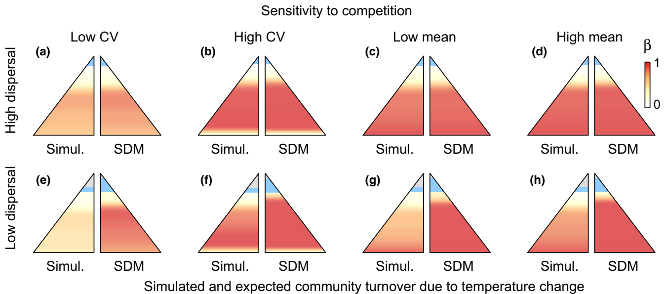
FIGURE 4 Temporal community turnover along an elevational temperature gradient ( \beta -diversity, represented by the gradient from white to red, see legend in (d)) following climate warming. The left section of the mountains represents the results of simulations (“Simul.”), while the right section represents the expected turnover obtained by stacking species distribution models projection (“SDM”). Shown are eight scenarios that differ depending on dispersal ability (rows) and sensitivity to competition within the species pool (a, e: coefficient of variation [CV] = 0.1; b, f: CV = 1/\sqrt{3} ; c, g: mean = 0.7; d, h: mean = 1.5; a–d: d = 10^{-1} ; e–h: d = 10^{-4} ). In each panel, all other parameters except the ones specified in the header of their line and column were set to the average value of their respective distribution (see Table S1). The lowest elevation communities are not displayed (see Appendix S1). Communities at the highest elevations resulting from colonization of previously unoccupied habitat are coloured in blue, while communities that remain empty despite warming are in light grey. Note that outcomes of temporal community turnover obtained from stacking SDM projections can also differ slightly among panels due to different initial conditions (i.e. initial burn-in period that allowed the meta-communities to equilibrate) [Colour figure can be viewed at wileyonlinelibrary.com ]
